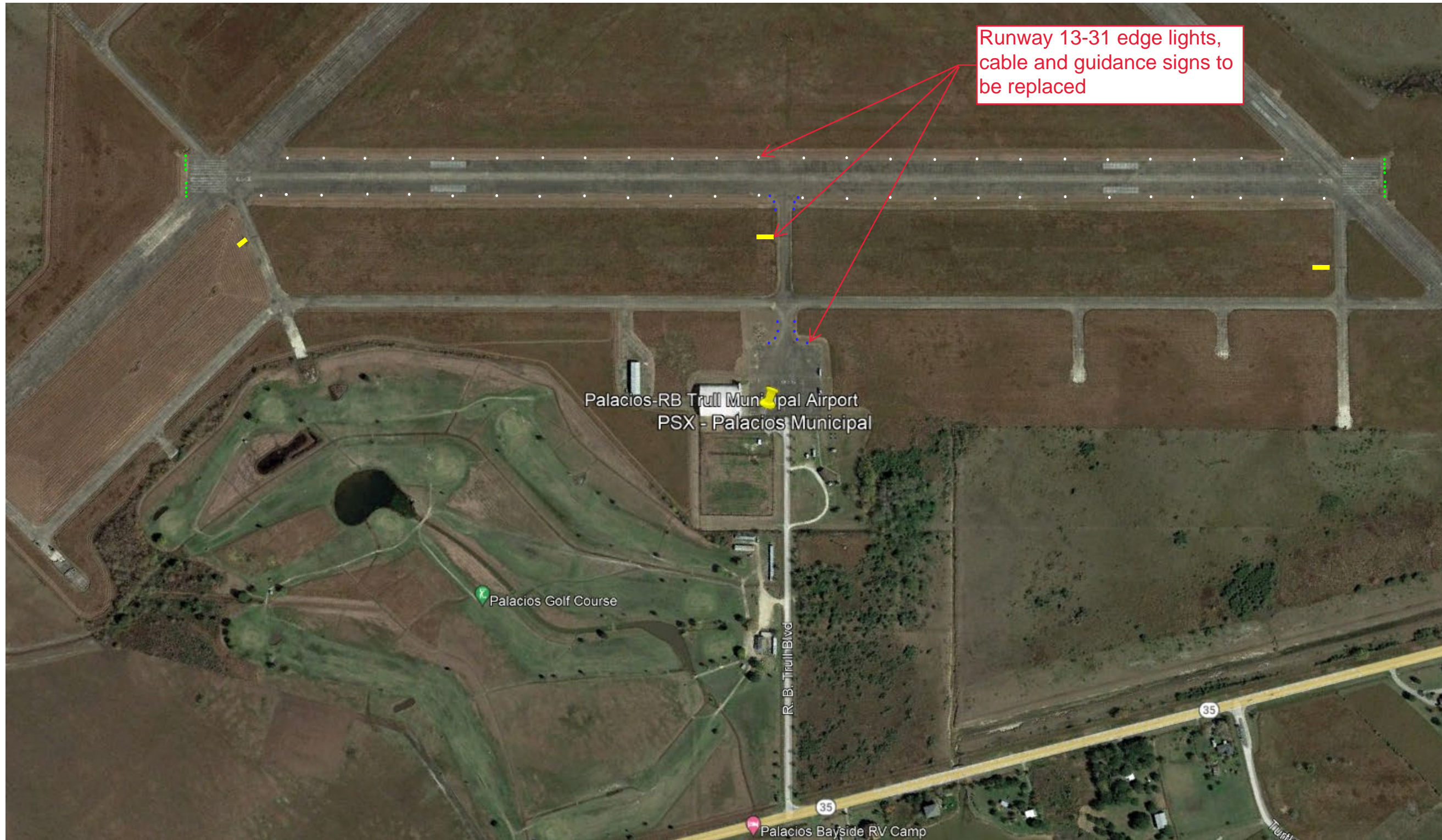
Palacios Municipal Airport (PSX) – Runway 13-31 Lighting Improvements
